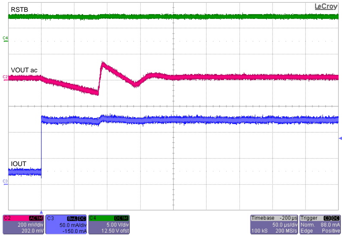
Figure 32. Detail of the 20 mA to 120 mA Transition at V_{IN} = 13\text{ V} and V_{OUT} = 5\text{ V}
