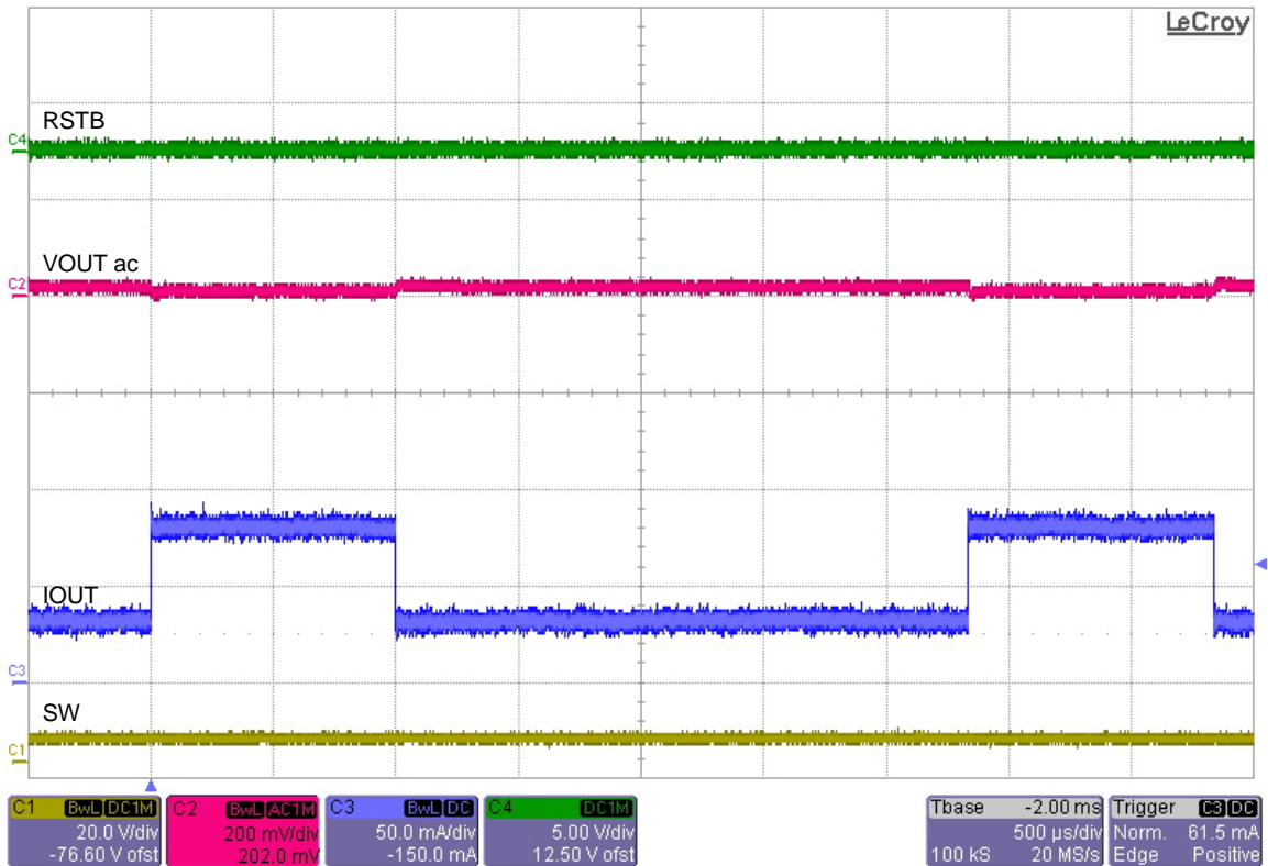
Figure 33. V_{IN} = 13\text{ V} , V_{OUT} = 5\text{ V} , 20 mA to 70 mA Load Transient – LDO Mode Only (no transition)
