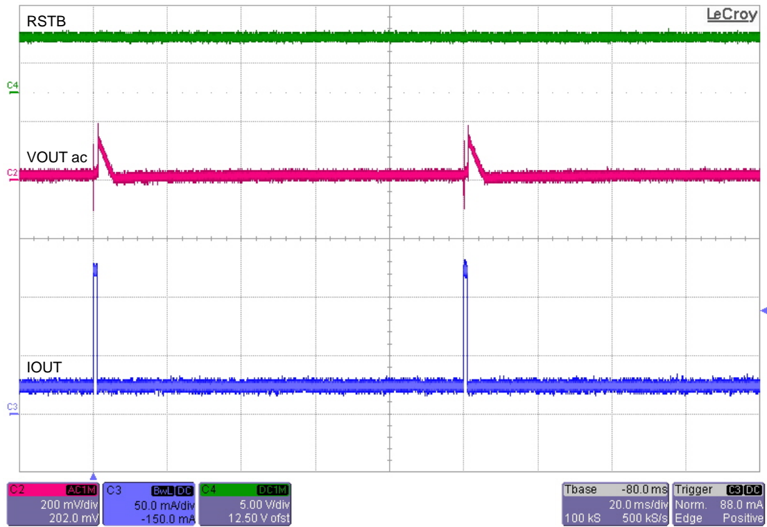
Figure 31. V_{IN} = 13\text{ V} , V_{OUT} = 5\text{ V} , 20 mA to 120 mA Load Transient – with Mode Transition
