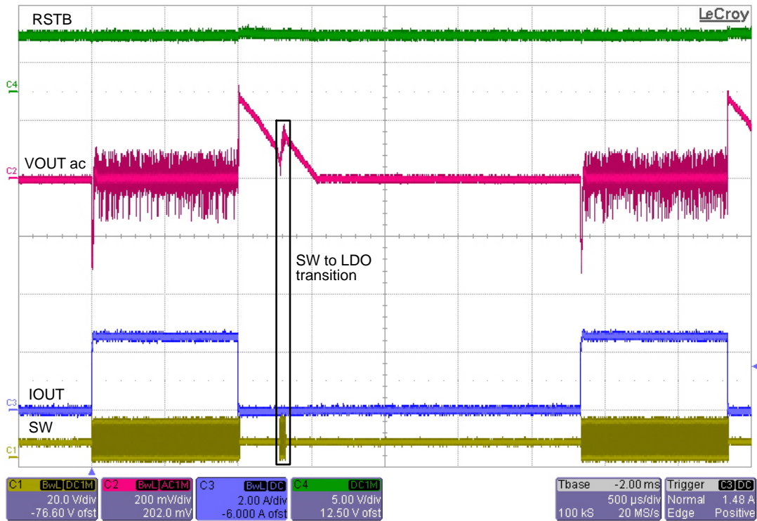
Figure 29. V_{IN} = 13\text{ V} , V_{OUT} = 5\text{ V} , 20 mA to 2.5 A at 1 A/μs – with Mode Transition
