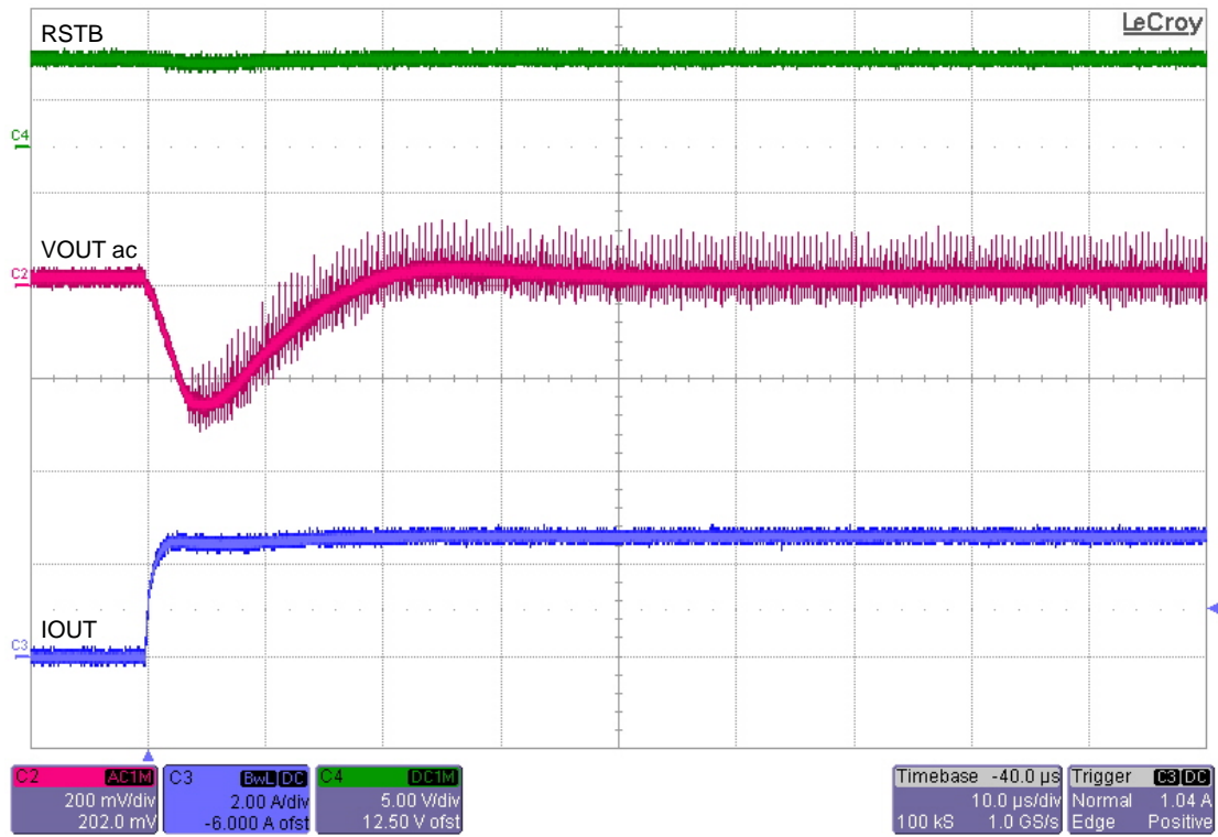
Figure 30. Detail of the 20 mA to 2.5 A Transition at V_{IN} = 13\text{ V} and V_{OUT} = 5\text{ V}
