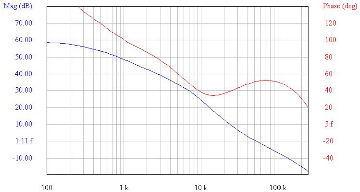
Figure 36. Bode Plot of the Open Loop Transfer Function of a Buck Converter using the NCV891330 for V_{in} = 13\text{ V} , V_{out} = 3.3\text{ V} , I_{out} = 2\text{ A} , C_{out}=3 \times 10\ \mu\text{F} and L=2.2\ \mu\text{H}
